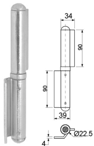
HINGE DEKKSON ES-IR 34X90-39X90 GALV Max Capacity : 100 kg / pair
