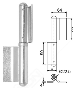
HINGE DEKKSON ES-IR 64X90-39X90 GALV Max Capacity : 100 kg / pair
